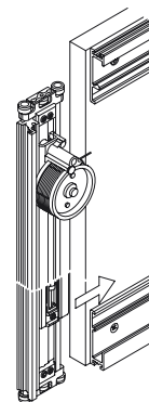
HAWA-Concepta 25/30.
