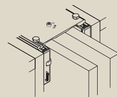
Connector 110 mm (4 11 / 32 ”): Recess for two pivot/slide-in doors.
