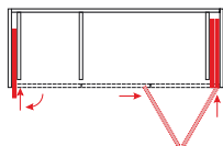
Combination 3-doors HAWA-Concepta 25/30/40/50 and HAWA-Folding Concepta 25
