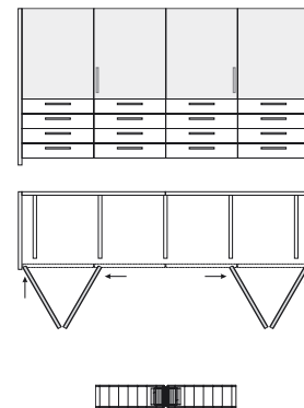
Door centring with magnetic centring elements.
