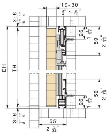
HAWA-Concepta 25/30.
