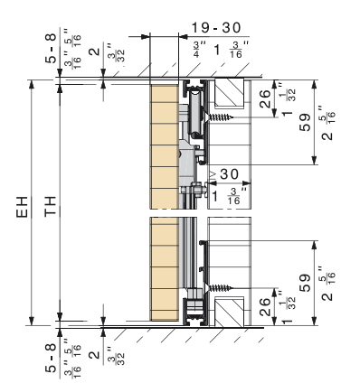
HAWA-Concepta 40/50.
