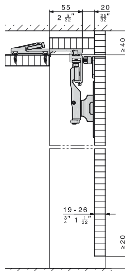
Door centring with magnetic centring elements.
