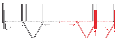
Additional combination options HAWA-Concepta 25/30/40/50 and HAWA-Folding Concepta 25
